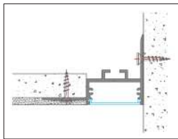
MONTAGGIO INCASSO CARTONGESSO FLUSH-MOUNTED PLASTERBOARD
