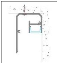
MONTAGGIO A PARETE WALL MOUNTED
